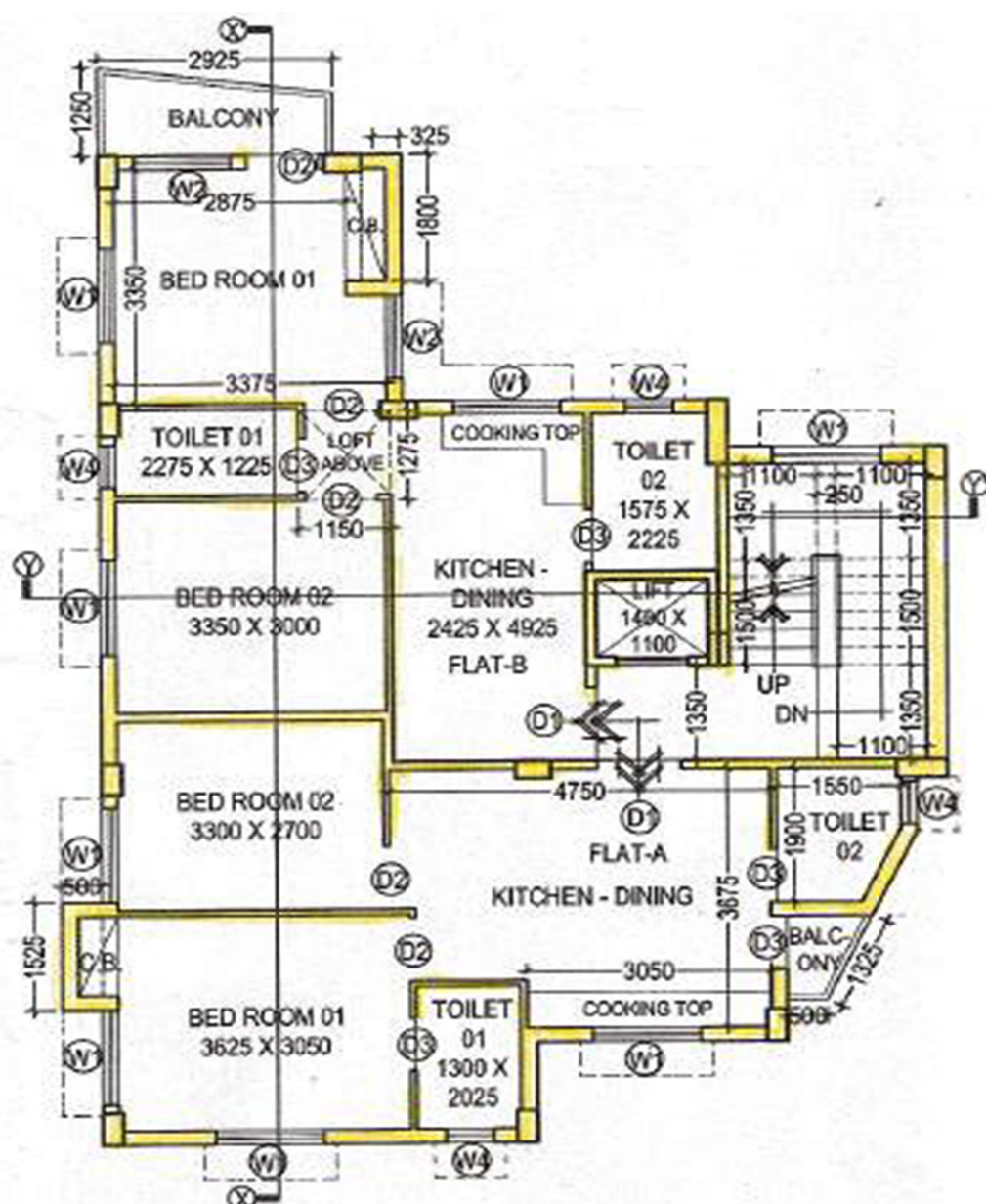
TYPICAL 1ST. & 2ND. FLOOR PLAN. SCALE : 1 :100
